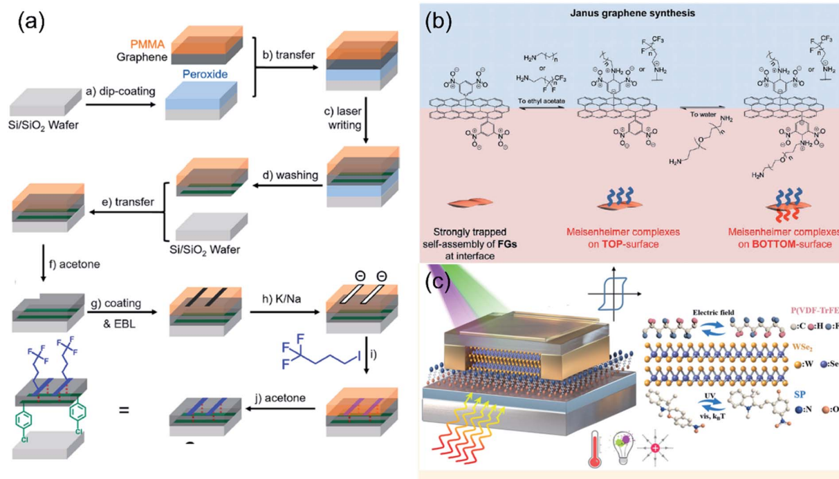
Fig. 2 Schematic representation of the three main strategies for the preparation of Janus 2DMs through an antarafacial binding of (macro) molecules. (a) Two-step functionalization assisted by a transfer approach, (b) functionalization of 2DM surfaces at liquid-liquid interfaces and (c) step by step procedure. (a) Adapted with permission from ref. 41, Copyright 2017 American Chemical Society. (b) FGs stands for functionalized graphenes. Adapted from ref. 43 with permission from Wiley-VHC. (c) Adapted with permission from ref. 52, Copyright 2017 American Chemical Society.
