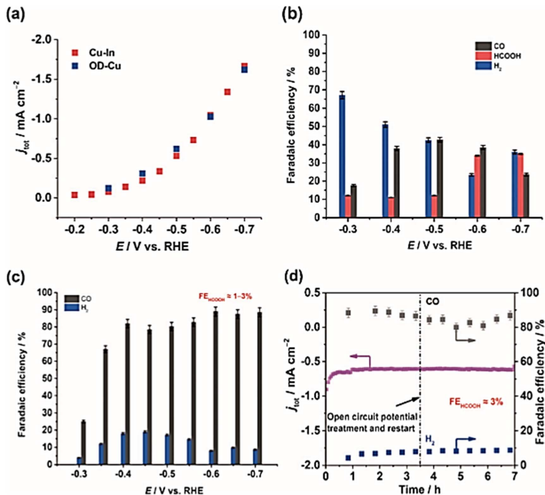
Fig. 6 (a) The current density of OD-Cu and Cu-In, (b) faradaic efficiencies of OD-Cu, (c) faradaic efficiencies of Cu-In, (d) test stability for the Cu-In catalyst at -0.6 V vs. RHE in 0.1 M KHCO 3 /CO 2 . Reproduced with permission. 77 Copyright ©2015, Wiley-VCH.
