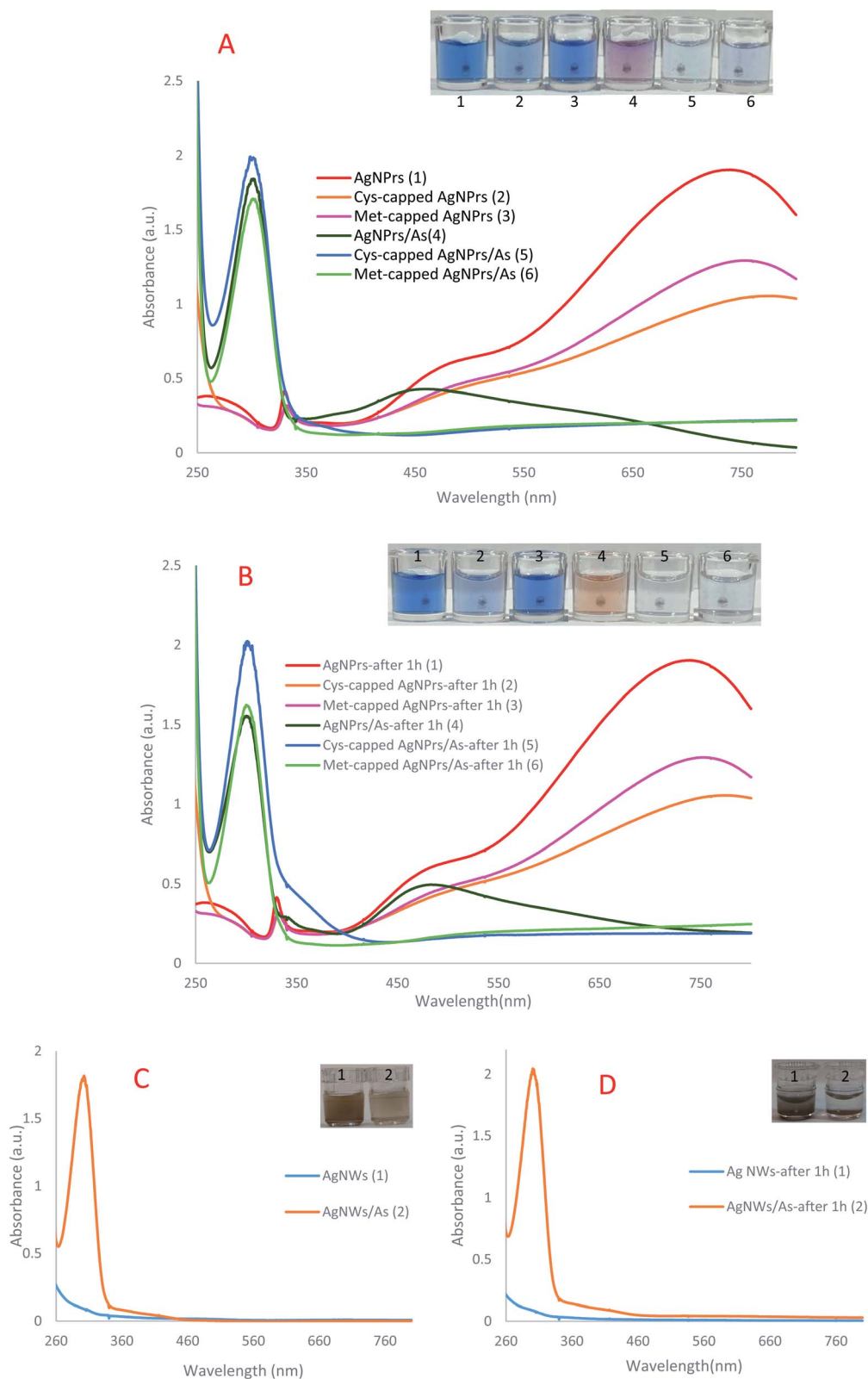
Fig. 1 The UV-Vis spectra of sensing probes in the presence and absence of arsenic (A) AgNPs, Cys-capped AgNPs, Met-capped AgNPs; (B) AgNPs, Cys-capped AgNPs, Met-capped AgNPs after 1 h; (C) AgNWs and (D) AgNWs after 1 h.
