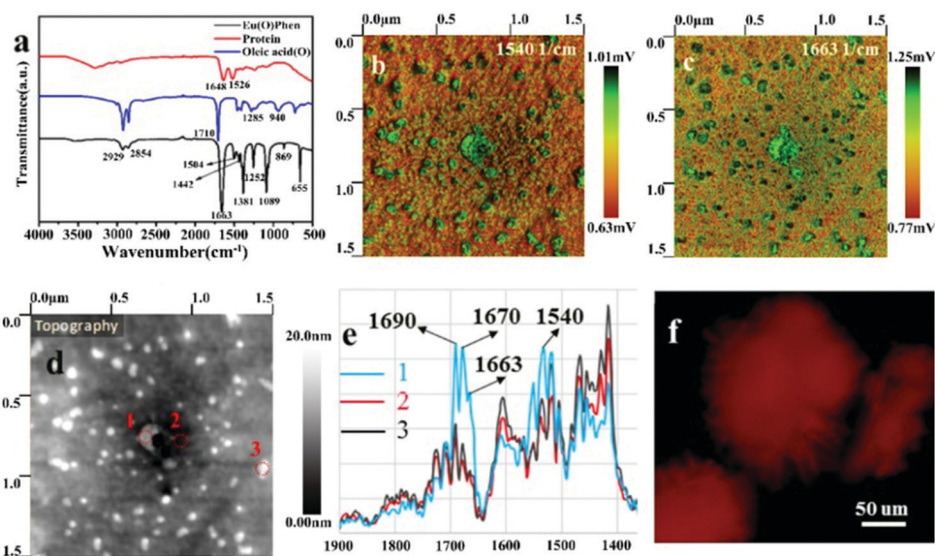
Fig. 11 The concentration of oleic acid used during nano-label synthesis was 0.05 \text{ mol L}^{-1} in FTIR spectra and PiFM images. (a) FTIR spectra of protein, oleic acid, and \text{O}^{\text{Eu}^{3+}}\text{Phen} complexes; PiFM images taken with laser tuned to (b) 1540 \text{ cm}^{-1} for protein and (c) 1663 \text{ cm}^{-1} for \text{O}^{\text{Eu}^{3+}}\text{Phen} complexes in the sample; (d) the detection points of the sample, overlaid on a topographical map; (e) PiFM infrared spectra for the detection points; (f) the fluorescence microscopy image of the sample. Reproduced from Zhao et al. 61
