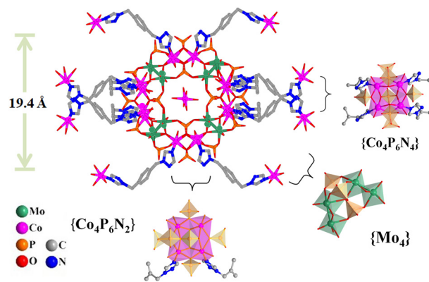
Fig. 1 Ball-stick representation of a wheel-shaped \{\text{Co}_{16}\text{Mo}_{16}\text{P}_{24}\} cluster in hybrid 1 . Color code: Co, purple; Mo, green; O, red; N, blue; and P, orange.
