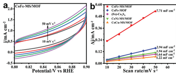
Fig. 5 (a) Cyclic voltammograms of the CoFe-MS/MOF. (b) Double layer currents of different catalysts versus the scan rate.
