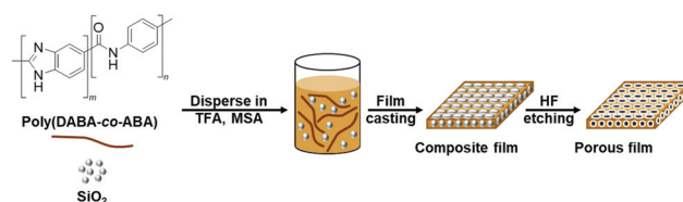
Fig. 1 Preparation of porous poly(DABA-co-ABA) films.
