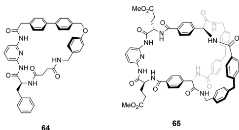
Fig. 24 Macrocyclus 64 and 65.
