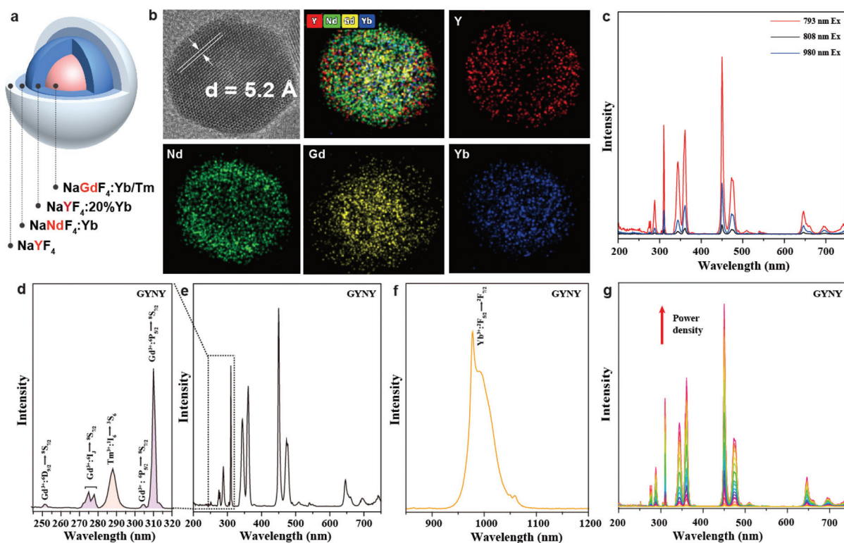
Fig. 1 (a) Schematic illustration of a \text{NaGdF}_4\text{:}49\%\text{Yb},1\%\text{Tm}@ \text{NaYF}_4\text{:}20\%\text{Yb}@ \text{NaNdF}_4\text{:}10\%\text{Yb}@ \text{NaYF}_4 (GYNY) nanoparticle. (b) High-resolution TEM image and elemental mapping of the corresponding GYNY nanocrystal. (c) Corresponding upconversion luminescence spectra of GYNY nanoparticles in cyclohexane under 793, 808 and 980 nm excitation at a power density of 28.0 \text{ W cm}^{-2} . (d–f) Room-temperature luminescence spectra in the range of 240–750 nm and 850–1200 nm of GYNY nanoparticles in cyclohexane. (g) Excitation-power-dependent upconversion emission spectra of GYNY nanoparticles under 793 nm excitation.
