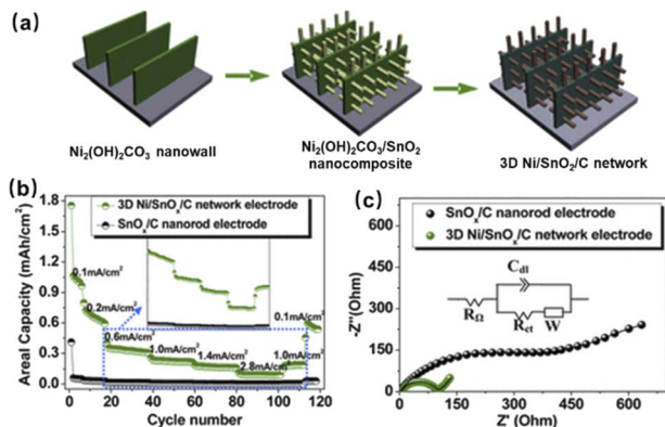
Fig. 11 (a) Fabrication process, (b) rate performance and (c) EIS plot of the 3D Ni/SnO 2 /C electrode. Reproduced with permission from ref. 81, Copyright© 2013, American Chemical Society.
