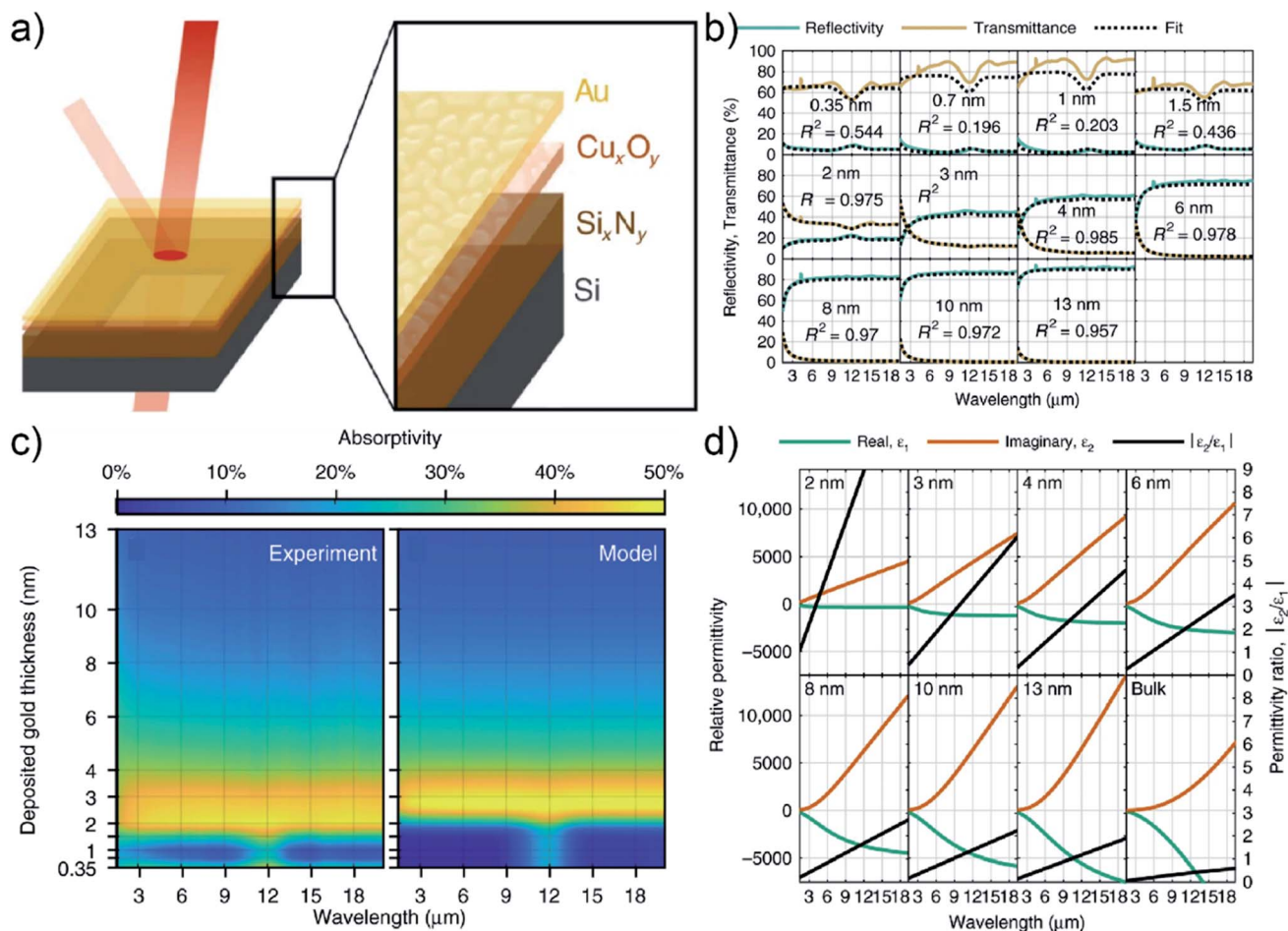
Fig. 11 (a) Scheme of fabricating UTGLs with Cu x O y seed layer and Si 3 N 4 support layer. (b) Measured transmittance (khaki lines) and reflectivity (green lines) of UTGLs with different thicknesses, as well as the fitted results (black dash lines) based on the Drude model. (c) Mappings of measured and modelled absorptivity as a function of deposited Au thickness and wavelength. (d) Relative permittivity of UTGLs with different thicknesses. The real part \epsilon_1 , imaginary part \epsilon_2 , and the permittivity ratio |\epsilon_2/\epsilon_1| were presented by orange lines, green lines, and black lines, respectively. Reproduced with permission. 102 Copyright the authors.
