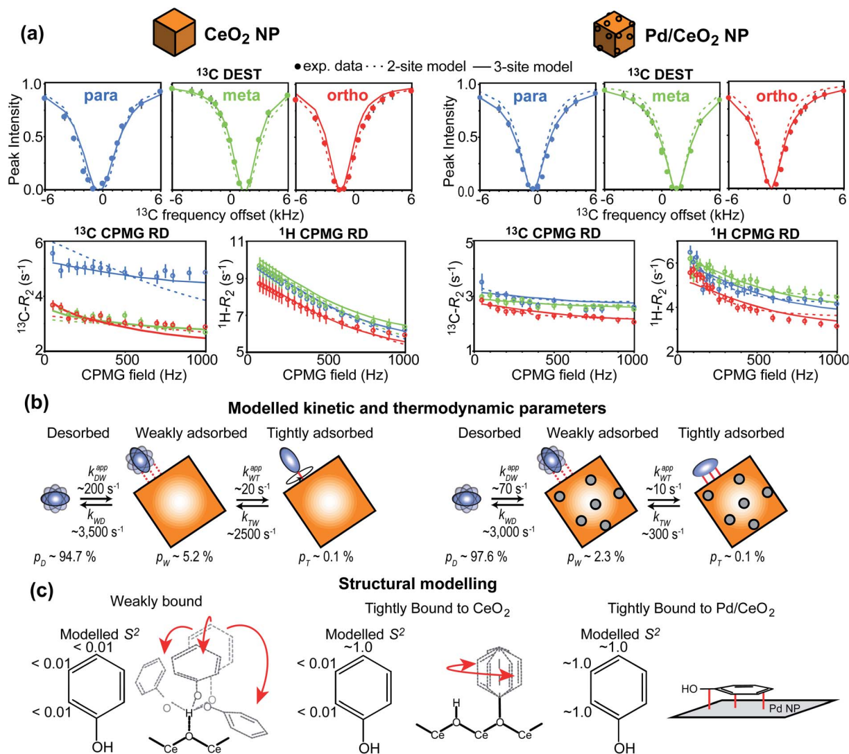
Fig. 13 Combined analysis of ^{13}\text{C} R_1 , ^{13}\text{C} R_2 , ^{13}\text{C} DEST, and ^1\text{H} and ^{13}\text{C} CPMG RD experiments on the PhOH-Pd/CeO 2 system. (a) ^{13}\text{C} DEST (saturation field strength = 1 kHz) and ^1\text{H} and ^{13}\text{C} CPMG RD profiles of PhOH in the presence of 1 wt% CeO 2 (left) and 1 wt% Pd/CeO 2 (right) NPs. Data were collected at 800 MHz. Experimental data for the para , meta , and ortho C-H bonds are represented in blue, green, and red circles, respectively. The dotted and solid lines represent the best fit to a two-site and three-site exchange model, respectively. (b) Modelled kinetic and thermodynamic parameters for PhOH adsorption on CeO 2 (left) and Pd/CeO 2 (right) NPs. PhOH is a blue oblate, CeO 2 is an orange square, and Pd sites are gray spheres. (c) Structural modelling of PhOH adsorbed on the CeO 2 and Pd/CeO 2 surface. The order parameter ( S^2 ) obtained for each C-H group is shown. Adapted from Egner et al. 192
