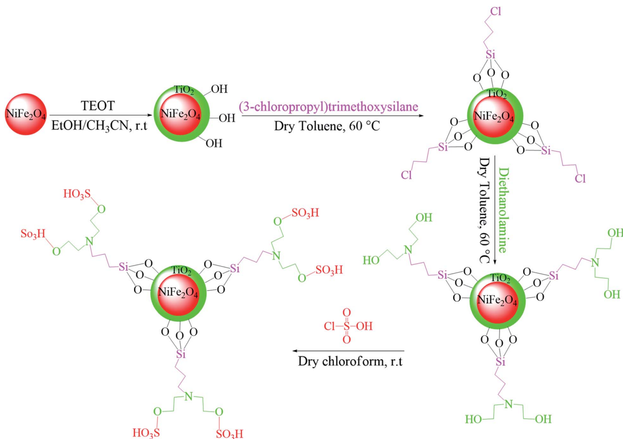
Fig. 7 Approach for the preparation of the \text{NiFe}_2\text{O}_4 @ \text{TiO}_2 - \text{SiO}_2 -Pr-DEA- \text{OSO}_3\text{H} nanocatalyst (r.t.: room temperature). This figure was adapted with permission from Chem. Sel. , 2019, 4, 17–23. 71
