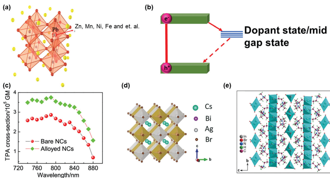
Fig. 14 (a) Crystal structure of doped APbX 3 lead halide perovskites. (b) Schematic showing the mid-gap states arising due to doping in APbX 3 halide perovskites. (c) Wavelength-dependent TPA cross-sections of CsPbI 3 perovskite NCs (pure and doped with Zn 2+ ). (d) Crystal structure of lead-free double-perovskite Cs 2 AgBiBr 6 viewed along the a -axis. (e) Crystal structure of lead-free zero-dimension perovskite (C 4 H 14 N 2 ) 2 In 2 Br 10 viewed along the a -axis. The organic cations intercalate between the isolated polyhedrons. (a) and (c) Reprinted with permission from ref. 121. Copyright 2020 American Chemical Society. (b) Reprinted with permission from ref. 123. Copyright 2019 American Chemical Society. (d) Reprinted with permission from ref. 124. Copyright 2018 Wiley-VCH Verlag GmbH & Co. KGaA, Weinheim. (e) Reprinted with permission from ref. 125. Copyright 2019 Wiley-VCH Verlag GmbH & Co. KGaA, Weinheim.
