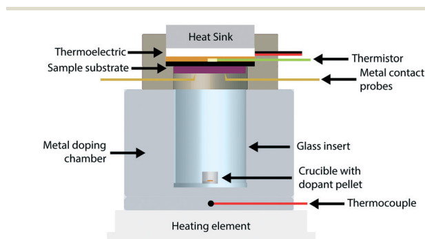
Fig. 1 Cross section of apparatus for vapor doping experiments. Metal doping chamber houses glass insert with alumina crucible and F4TCNQ pellet within. F4TCNQ pellet is vaporized by heating the metal doping chamber to a desired temperature on a hot plate, whose temperature is monitored by a thermocouple in the base. The sample is simultaneously measured and held stable by the metal contact probes, and a thermoelectric holds the temperature of the sample to a set constant from 0 °C to 70 °C. All vapor doping experiments were performed in an argon glovebox.
