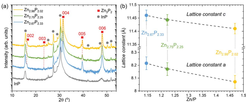
Fig. 2 Structural analysis of the monocrytalline zinc phosphide thin films. (a) XRD patterns of three monocrytalline zinc phosphide thin films with various Zn/P compositions, along with the XRD pattern of the bare InP substrate measured under the same conditions. Gray circles denote reflections corresponding to the InP substrate, while red squares denote reflections belonging to the tetragonal structure ( P4_2/nmc ) of zinc phosphide. (b) Compositional dependence of the lattice constants a and c calculated from the XRD and SAED measurements.
