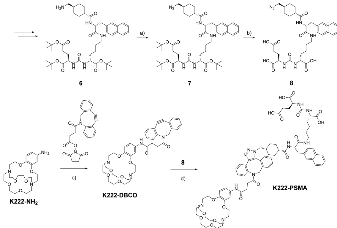
Scheme 2 Synthetic route towards K222-DBCO and K222-PSMA Reaction conditions: (a) \text{FSO}_2\text{N}_3 , 3 \text{ M KHCO}_3 , \text{MTBE/DMF/H}_2\text{O} , r.t., 5 min; (b) \text{TFA} , \text{DCM} (1 : 2), r.t., 3 h; (c) \text{DBCO-NHS} , \text{DMF} , r.t., overnight; (d) 8 , \text{DMF/MeOH} (1 : 1), r.t., overnight.
