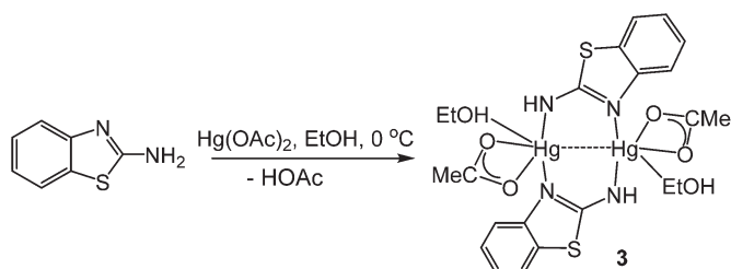
Scheme 2 Formation of 3 from reaction of abt and \text{Hg}(\text{OAc})_2 at 0^\circ\text{C} .
