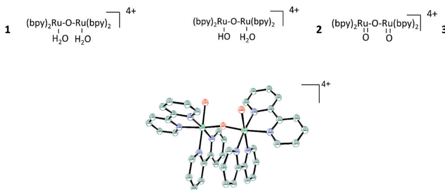
Fig. 118 Molecular structure of cis,cis -[(bpy) 2 Ru(H 2 O)Ru III O(OH 2 )-(bpy) 2 ] 4+ ( 1 ). 1477 Reprinted with permission from ref. 1477 Copyright 1985. American Chemical Society.
