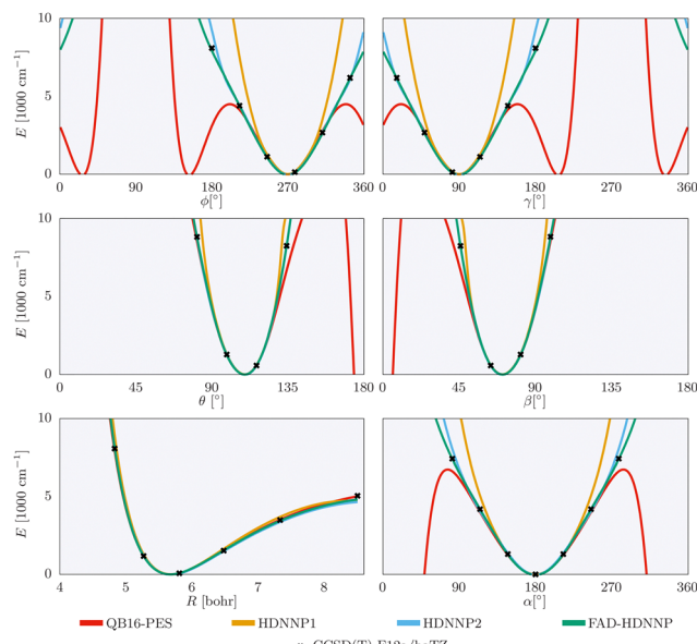
Fig. 4 1-dimensional cuts of the three investigated HDNNPs and the QB16 potential along the intermolecular coordinates ( cf. Fig. 1) of the formic acid dimer used in the reduced-dimensionality variational computations.
