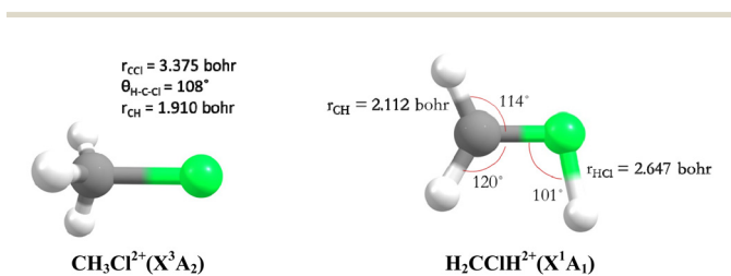
Fig. 1 C_{3v} (left) and planar (right) stable forms of chloromethane doubly charged ions as computed by Duflot et al. 22,23 and confirmed presently at the RCCSD(T)/aug-cc-pVTZ level.
