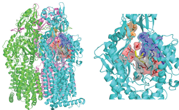
Fig. 2 MexB structure: the left panel highlights L, T, and O monomers of MexB colored in green, cyan, and magenta, respectively (PDB Id: 3W9J29). The detailed visualization on the right shows the different DP T sub-regions of MexB considered in this work: the interface is colored in gray (residues S79, T91, K134, F573, F617, M662, and E673), the cave is colored in red (residues Q46, T89, T130, N135, F136, V139, Q176, K292, Y327, V571, R620, and F628) and the groove is colored in blue (residues K151, F178, G179, R180, D274, S276, I277, A279, S287, P326, F610, V612, F615, and V47; S48, Q125, G126, R128, Q163, D174, F175, and Q273 that are located near the exit gate, colored in orange). The switch loop is represented as a yellow cartoon.
