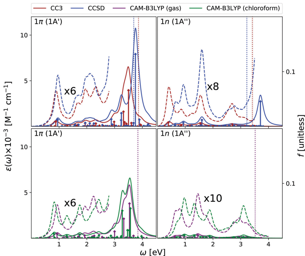
Fig. 5 Cytosine. Upper panels: ESA at EOM-CCSD/aug-cc-pVDZ and EOM-CC3/aug-cc-pVDZ levels of theory in gas phase. Bottom panels: ESA at TD-CAM-B3LYP/aug-cc-pVDZ level of theory in gas phase and in chloroform solution. The spectra in dashed line have been enhanced by the factor indicated. Geometry optimized in the gas phase enforcing C_s symmetry. The vertical lines indicate the first ionisation energy in the gas phase ( \Delta SCF at DFT level). HWHM = 0.0045563 hartree.
