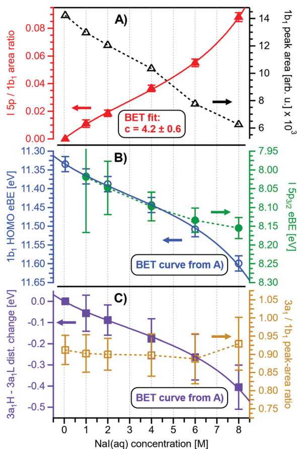
Fig. 2 Results for NaI (aq) solutions extracted from fits to the spectra plotted as a function of salt concentration (bottom axis). (A) Solute I − 5p peak area normalized by the 1b 1(0) peak area in red (full triangles; left axis) and absolute 1b 1(0) peak area in black (open triangles; right axis). The I − 5p peak successively increases in relative intensity while the liquid-water features (represented by the 1b 1 intensity) diminish due to reduced relative concentration and enhanced scattering in the surface layer. No saturation behavior is observed for the NaI solute, and instead the trend rather steepens at concentrations above 4 M. A BET (Brunauer, Emmett, and Teller) isotherm was fitted to the data (red line), which yields an excellent agreement with the experimental results (see text for details). (B) Electron binding energy (eBE) of water's 1b 1(0) peak in blue (open circles; left axis) and the I − 5p peak in green (full circles; right axis). Both features shift slightly towards higher eBEs by the same amount but deviate somewhat towards very high concentrations. The 1b 1(0) peak eBE follows the surface enrichment of I − 5p 1:1, which is apparent from the excellent match to the BET curve (reproduced here as blue curve by shifting and scaling the red fit curve from panel A). In case of the saturation-like behavior of the I − 5p peak, it can be assumed that the large surface enrichment above 4 M concentration significantly diminishes the solvation of I − , which partly compensates the increase in eBE. (C) Change in energetic splitting of the 3a 1 double peak in purple (full squares; left axis) and 3a 1 /1b 1 peak-area ratio in orange (open squares; right axis). The overall peak splitting decreases rapidly with increasing concentration while the peak-area ratio stays constant, i.e., the 3a 1 feature only seems to increase in relative height because of the diminishing peak distance. Again, the BET curve was reproduced in purple for comparison. The observed narrowing of the 3a 1 -peak split is in excellent agreement with the values of ref. 8.
