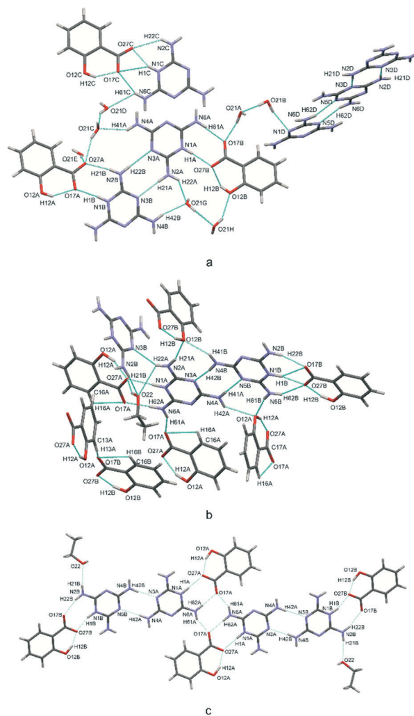
Fig. 2 Labelling schemes of all molecular components of cocrystals (I) and (II). Anisotropic displacement parameters of non-hydrogen atoms are drawn as ellipsoids with a 50% probability level.
