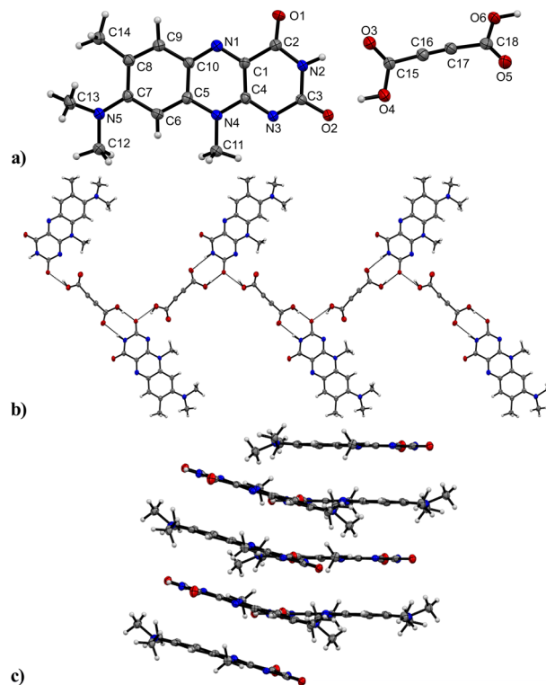
Fig. 4 Crystal structure of R:A . a) Asymmetric unit of R:A . Labels for H-atoms are omitted for clarity. View along the crystallographic a axis. b) Zig-zag chains formed by O–H···O and N–H···O interactions between A and R along the b axis. View along the a axis. c) Tilted \pi\cdots\pi stacks of R molecules. A removed for clarity. View along the b axis.
