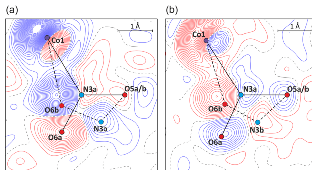
Fig. 4 Photodifference Fourier maps showing (a) the build-up of the endo -nitrito isomer after 1st irradiation (470 nm, F^{1st, ON} - F^{OFF} map), and (b) partial return of the system to the nitro form after 2nd irradiation (660 nm, F^{2nd, ON} - F^{1st, ON} map) (contours at 0.2 e Å -1 intervals, blue lines – positive values, red – negative; refined geometries of nitro forms – solid black lines, endo -nitrito forms – dashed black; for the map definition see the ESI†).
