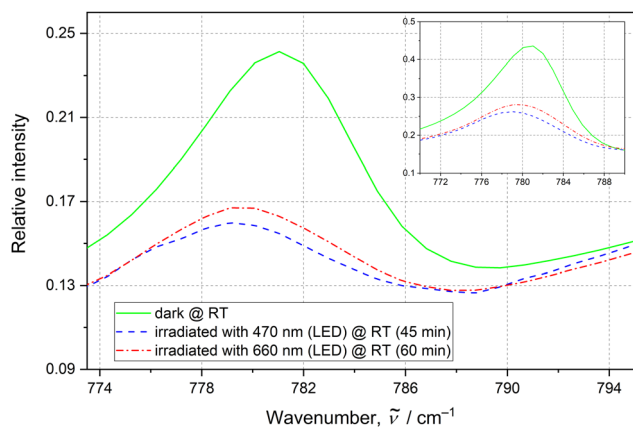
Fig. 3 The 781 cm -1 IR band, attributed to the \delta(\text{NO}_2) scissoring vibration, indicating switching. The RT spectra are recorded before any irradiation (green solid line), after 470 nm LED irradiation (blue dashed line) and after final 660 nm LED irradiation (red dotted-dashed line). The inset plot shows the same peak and its behaviour when irradiated with the 476 nm laser light (1 h), and then with the 556 nm laser light (1.5 h).
