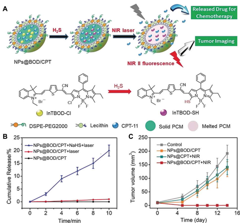
Fig. 7 NSFA-based activatable nanoparticles for imaging-guided cancer therapy. (A) Schematic illustration showing H 2 S-mediated in situ generation of photothermal transducers for cancer imaging and on-demand drug release. (B) Cumulative release profiles of CPT-11 from NP@BOD/CPT after various treatments. (C) Tumor growth curves of HCT116 tumor-bearing mice in various groups. Reproduced from ref. 114 with permission from Wiley-VCH.
