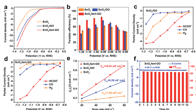
Fig. 3 (a) LSV curves (a) of \text{SnO}_2 , \text{SnO}_2/\text{GO} and \text{SnO}_2/\text{tert-GO} at a scan rate of 10\text{ mV s}^{-1} . (b) Faradaic efficiencies of formate when using \text{SnO}_2 , \text{SnO}_2/\text{GO} and \text{SnO}_2/\text{tert-GO} . (c and d) The partial current densities of formate, CO and \text{H}_2 of \text{SnO}_2/\text{GO} and \text{SnO}_2/\text{tert-GO} . (e) ECSA of \text{SnO}_2 , \text{SnO}_2/\text{GO} and \text{SnO}_2/\text{tert-GO} , where j_a and j_c are the anodic and cathodic current density, respectively. (f) The durability test of \text{SnO}_2/\text{tert-GO} at -0.96\text{ V vs. RHE} . All the tests were done in \text{CO}_2 -saturated 0.1\text{ M KHCO}_3 aqueous solution.
