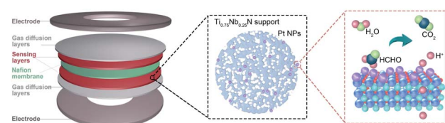
Fig. 1 Structure and performance characteristics of the proton exchange membrane fuel cell (PEMFC) gas sensor. Left: schematic illustration of the PEMFC sensor. Middle: microstructure of the sensing layer of the working electrode. Right: gas sensing at the working electrode (take formaldehyde detection as an example).
