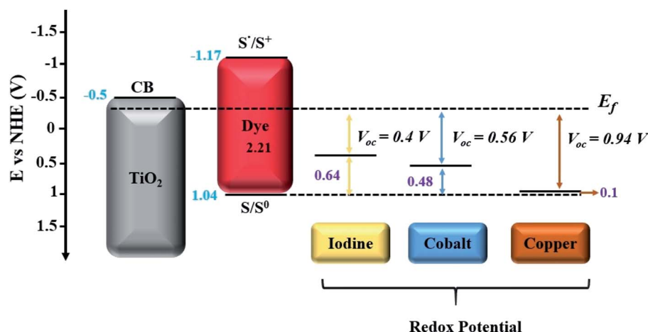
Fig. 5 Energetics in DSSCs with respect to redox potentials of each redox couple ( \text{I}^-/\text{I}_3^- , [\text{Co}(\text{bpy})_3]^{2+/3+} and [\text{Cu}(\text{dmp})_2]^{1+/2+} ) utilized in DSSCs. 55
