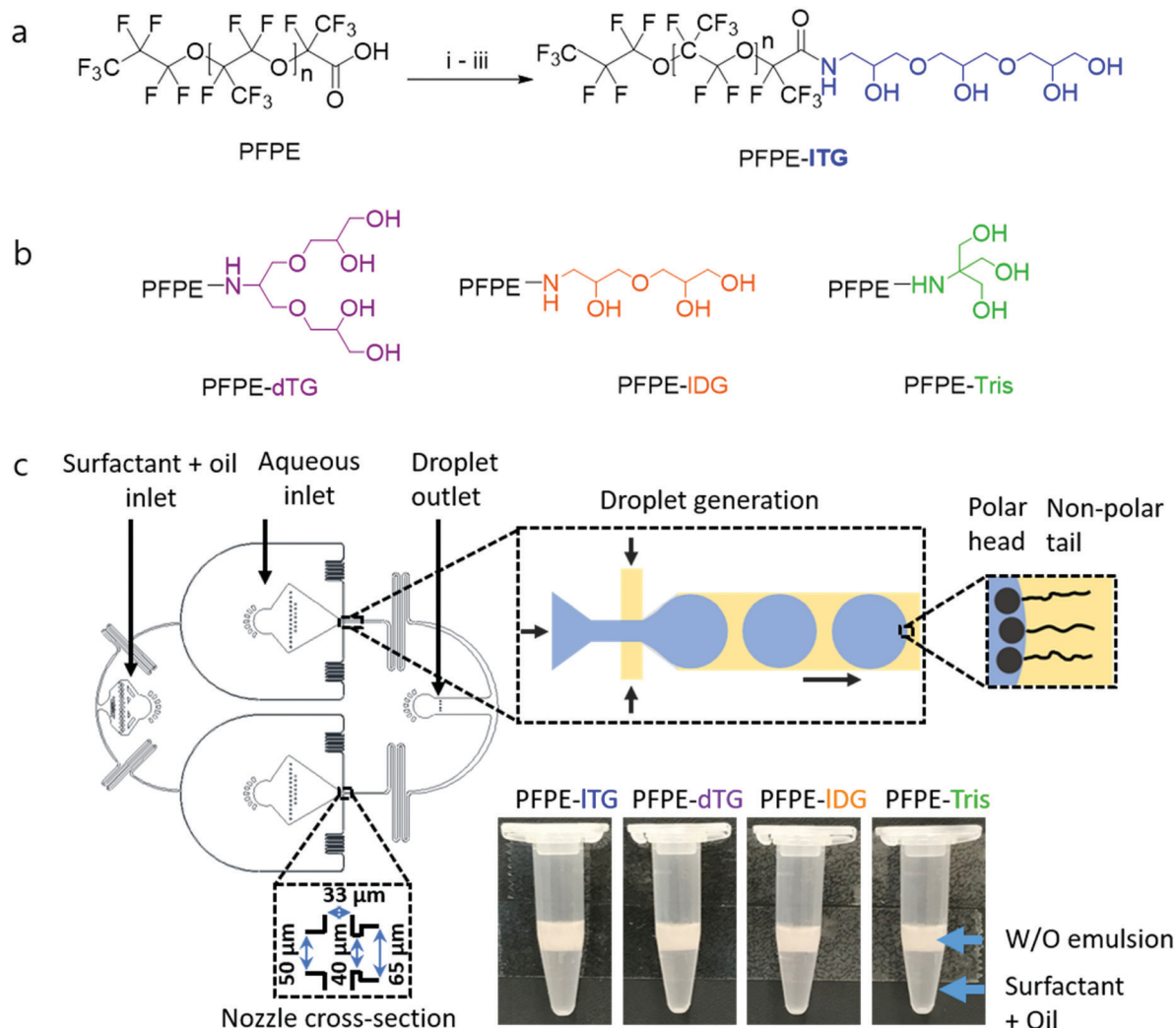
Fig. 1 (a) Synthetic approach to linear triglycerol fluorosurfactant through amide coupling: (i) (\text{COCl})_2 , HFE7100, cat. DMF, rt, overnight; (ii) acetal protected linear triglycerol-NH 2 , TEA, rt, overnight; and (iii) H + , CH 3 OH-HFE7100, reflux, overnight. (b) Schematic illustration of the surfactants with different head groups. (c) A microfluidic approach for parallel droplet generation (left). Top insets show the droplet pinch-off at the nozzle area and the orientation of the perfluoropolyether-based surfactant molecules at the interface of water (light blue) and oil (yellow). The polar head groups are shown using black circles and the non-polar tail groups are shown using black wavy lines. Dimension of the nozzle cross-section is shown on the bottom left inset. The height of the channel was 50 μm. The 15 mm long serpentine after the nozzles were used to allow the surfactant molecules to better adsorb at the water–oil interface. A further detail of a microfluidic setup and a parallel droplet making PDMS chip are shown in Fig. S1, ESI†. The bottom right panel shows the droplet emulsions generated using surfactants with four different polar head groups. Emulsions were collected in Eppendorf tubes where the white layer contains the emulsion droplets, and the residual surfactant solution (transparent) remains below the emulsion layer because of the high density of HFE7500 oil ( \rho = 1.614 \text{ g mL}^{-1} ).
