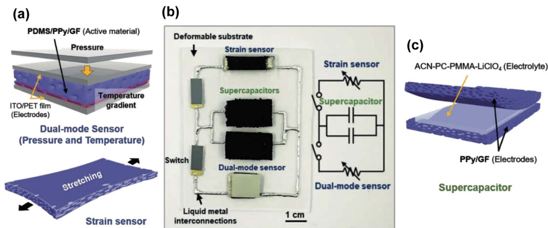
Fig. 3 (a) Schematic drawing of a pressure/temperature sensor and a strain sensor based on polypyrrole/graphene-foam material. (b) Picture showing the electric circuit connecting these elements with two supercapacitors using liquid metal interconnects. (c) Schematic drawing of the PPy/GF sandwich supercapacitor. Reproduced with permission of ref. 106. Copyright 2018 Wiley-VCH Verlag GmbH & Co. KGaA, Weinheim.
