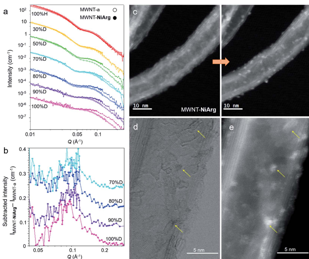
Fig. 5 SANS and STEM evidence of an organized distribution of NiArg on MWNT. (a) SANS profiles of MWNT-a (circles) and MWNT- NiArg (dots) in solvents of % D 0, 30, 50, 70, 80, 90 and 100. Data at successive % D are down-shifted by a factor of 0.1 for clarity. (b) SANS profile of MWNT- NiArg subtracted by the corresponding SANS profile of MWNT-a for % D 70, 80, 90 and 100%, showing a repeatable peak centered at 0.095 \text{ \AA}^{-1} . Successive plots are down-shifted by an increment of 0.08 for clarity. (c) Successive STEM-HAADF images of MWNT- NiArg at first scan and after exposure to electron beam. (d, e) Simultaneously recorded BF (d) and HAADF (e) STEM images of the same detail of MWNT- NiArg after beam exposure, showing co-localization (arrows) of MWNT structural defects (d) and Ni-rich clusters (e).
