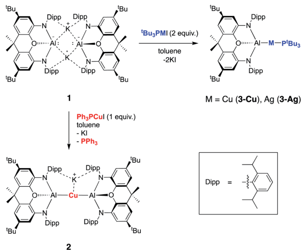
Scheme 1 Synthesis of aluminium–silver and aluminium–copper complexes 2, 3-Cu and 3-Ag from potassium alumynyl complex 1 via salt metathesis.
