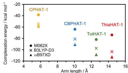
Fig. 8 Complexation energy–linker length plot of CPHAT-1 , CBPHAT-1 , ToIHAT-1 , and ThiaHAT-1 , calculated at the B3LYP-D3/6-311G(d,p), M062X/6-311G(d,p) and wB97XD/6-311(d,p) levels with the counterpoise method for BSSE correction.
