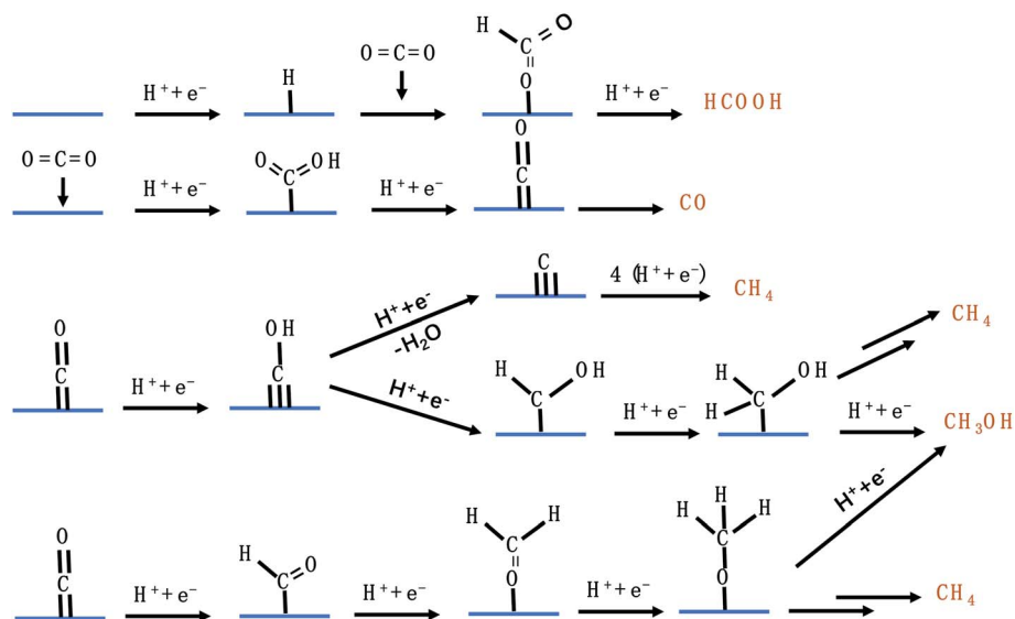
Fig. 4 The possible \text{CO}_2\text{RR} pathways for \text{C}_1 products.
