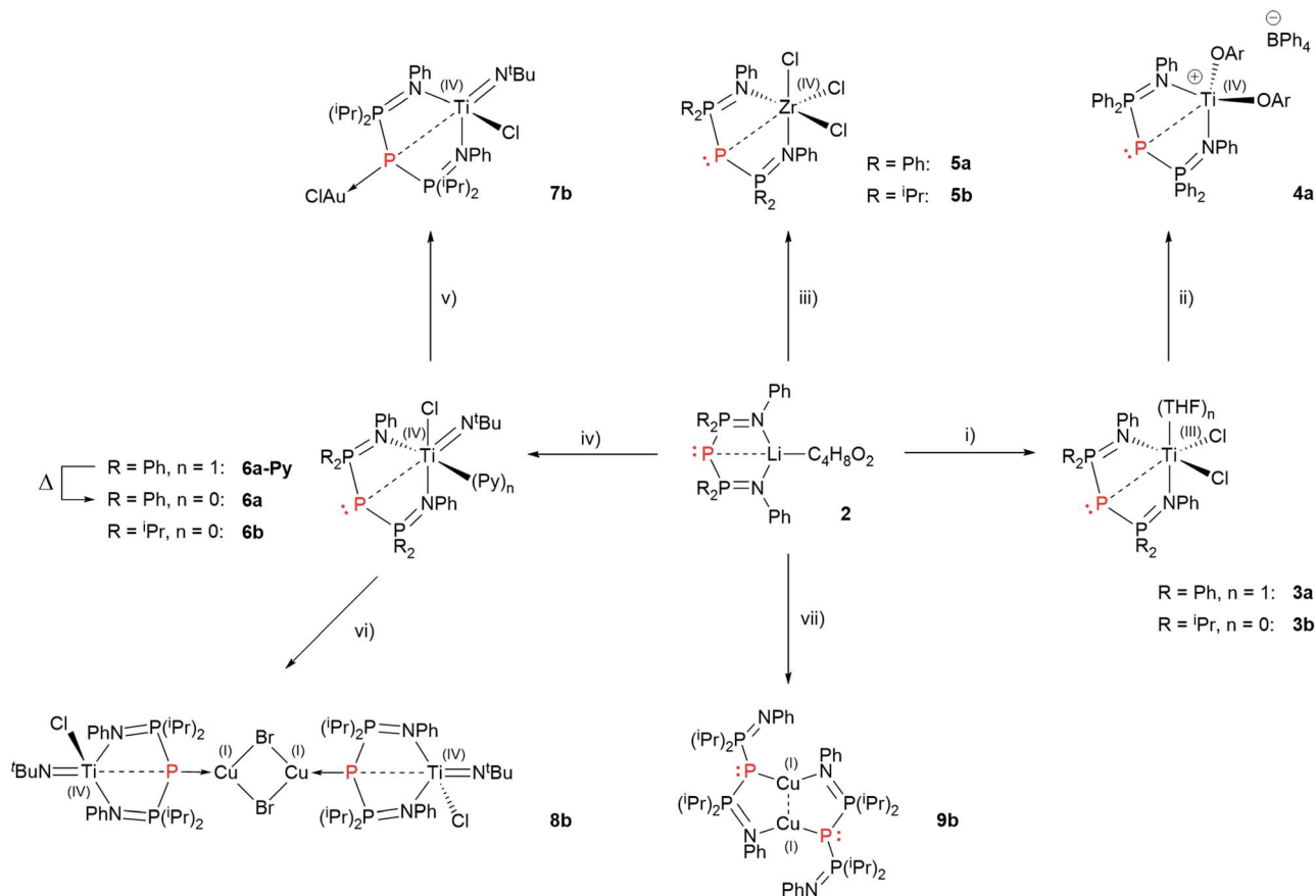
Scheme 6 Synthesis of group 4 and coinage metal complexes of BIPP. Reagents and conditions: (i) 1 eq. [\text{TiCl}_3(\text{THF})_3] , THF; (ii) 1 eq. [\text{ZrCl}_4] [\text{BPh}_4] , 2 eq. ArONa (OAr = 2,6-dimethylphenolato); (iii) 1 eq. \text{ZrCl}_4 , toluene; (iv) 1 eq. [\text{TiCl}_2(\text{N}^t\text{Bu})(\text{Py})_3] , toluene; (v) 1 eq. [\text{Au}(\text{THT})\text{Cl}] , \text{CH}_2\text{Cl}_2 ; (vi) 1 eq. CuBr, \text{CH}_2\text{Cl}_2 ; (vii) 1 eq. CuBr, toluene. All reactions were conducted at room temperature (THT = tetrahydrothiophene).
