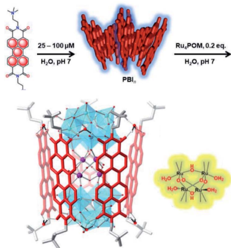
Fig. 19 A supramolecular dye-WOC assembly is formed in a 5 : 1 ratio when Ru-POM is added to \pi -stacked PBI in water. The Ru-oxo core of the POM is depicted besides the assembly. Used with permission from ref. 101.
