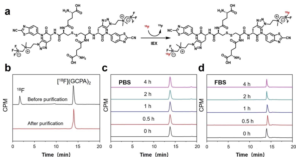
Fig. 1 (a) Radiosynthesis of ([\text{F}^{18}]\text{GCPA})_2 at 80 °C via the isotope exchange (IEX) method. (b) HPLC analysis of ([\text{F}^{18}]\text{GCPA})_2 before and after purification. (c and d) Stability assay of ([\text{F}^{18}]\text{GCPA})_2 in PBS and FBS.
