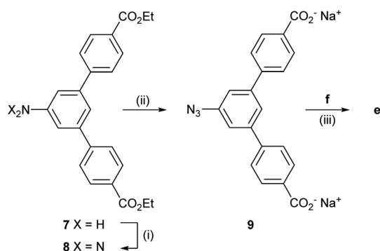
Scheme 4 Synthesis of the stopper 9 in 2 steps and CuAAC “click” reaction providing e . Reagents and conditions: (i) TMSN 3 , tBuONO, DMF, 0 °C to rt, 6 h, 98%; (ii) NaOH, THF–MeOH–H 2 O (4 : 4 : 1), 50 °C, 1 h, 86%; (iii) CuSO 4 ·5H 2 O, sodium ascorbate, H 2 O–MeOH (2 : 1), rt, 1 h, 65%.
