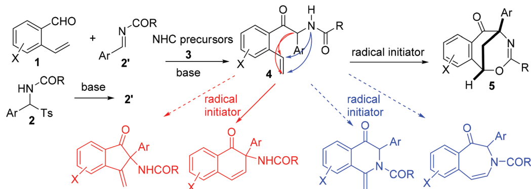
Scheme 1 Proposed NHC- and radical-mediated cascade reactions between o -vinyl benzaldehydes and N -acylarylimines.
