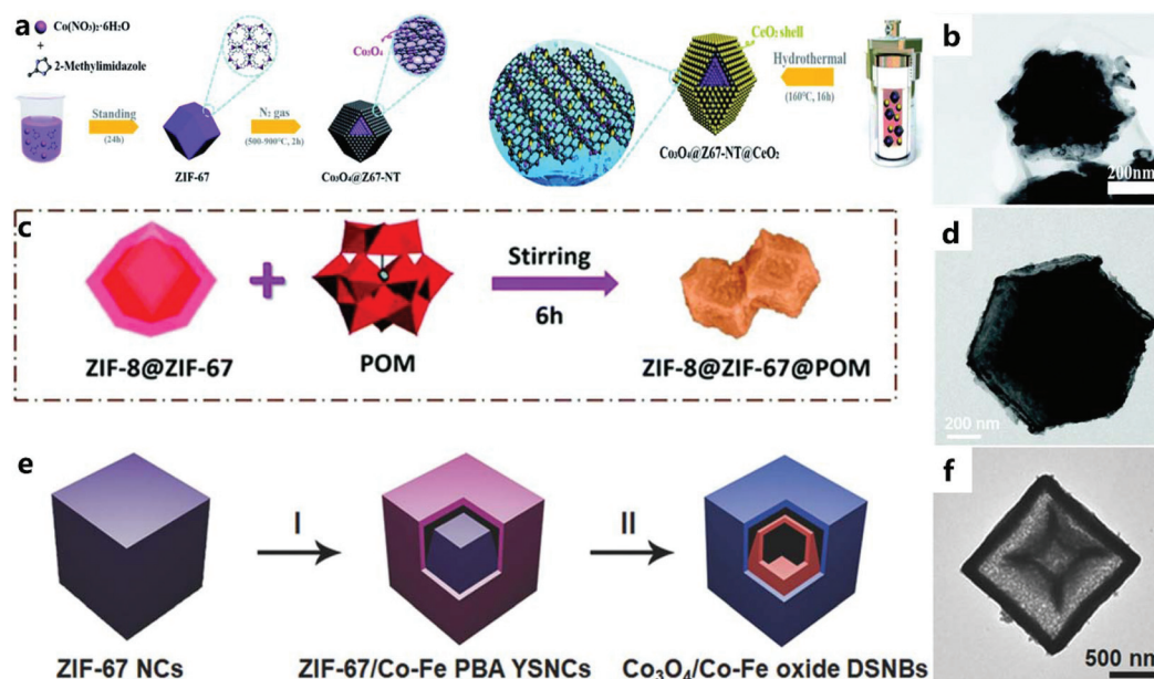
Fig. 4 (a) Synthesis route for the \text{Co}_3\text{O}_4@\text{ZIF-67-NT}@ \text{CeO}_2 composites. (b) TEM images of \text{Co}_3\text{O}_4@\text{ZIF-67-NT}@ \text{CeO}_2 . 68 Copyright © 2019, Royal Society of Chemistry. (c) Schematic diagram for the synthesis of \text{ZIF-8}@ \text{ZIF-67}@ \text{POM} . (d) TEM image of \text{ZIF-8}@ \text{ZIF-67}@ \text{POM} . 69 Copyright © 2019, Royal Society of Chemistry. (e) Schematic illustration of the formation process of \text{Co}_3\text{O}_4/\text{Co-Fe} oxide DSNBs. (f) TEM images of \text{Co}_3\text{O}_4/\text{Co-Fe} oxide DSNBs. 70 Copyright © 2018 Wiley-VCH Verlag GmbH & Co. KGaA, Weinheim.
