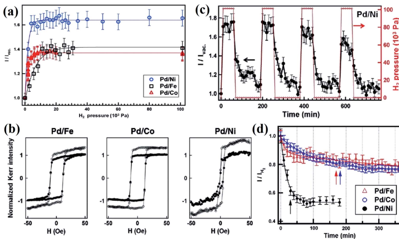
Fig. 9 (a) Normalized Kerr intensity as a function of \text{H}_2 pressure. The trend lines are included and do not represent the fitting curves. (b) The MOKE hysteresis loops measured in 1 \times 10^5 Pa \text{H}_2 (open circles) and a vacuum (filled circles). (c) Normalized Kerr intensity (left axis) measured with cycles of \text{H}_2 exposure (right axis) for the demonstration of reversibility. (d) Normalized Kerr intensity as a function of time, after \text{H}_2 is pumped out. The trend lines are included and do not represent the fitting curves. The arrows indicate the time constant when the Kerr intensity recovered 80% of the enhancement. Reprinted with permission from (58). Copyright (2013) Elsevier.
