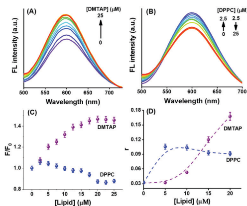
Fig. 3 Influence of the added GUVs from (A) DMTAP and (B) DPPC lipids on the fluorescence emission of the GSH-AuNCs in aqueous buffer under normal conditions ( \lambda_{\text{ex}} = 375 \text{ nm} ); (C) provides a comparative plot of the relative fluorescence yields due to the interactions and (D) shows the steady state fluorescence anisotropy ( r ) plots for the two cases (the dashed lines are to guide the view).
