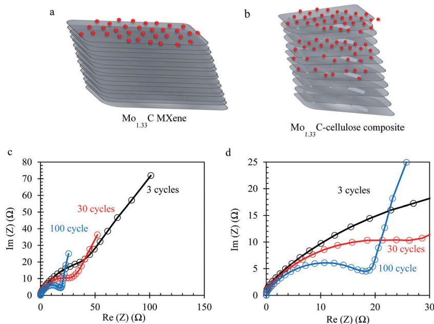
Fig. 5 (a) and (b) Schematic illustration of the ion transport during electrochemical cycling of the Mo 1.33 CT x MXene and the Mo 1.33 CT x -cellulose composite, respectively. The red balls represent the protons of the electrolyte, where the in-plane ion transport is hindered in the pristine MXene owing to the restacking of MXene sheets. (c) and (d) Nyquist plots of the H-Mo x C 5% Cel electrodes collected after 3rd (black), 30th (red) and 100th CV cycles at 10 mV s -1 , indicating the decrease in the charge transfer resistance and increase of ions transport upon electrochemical cycling.
