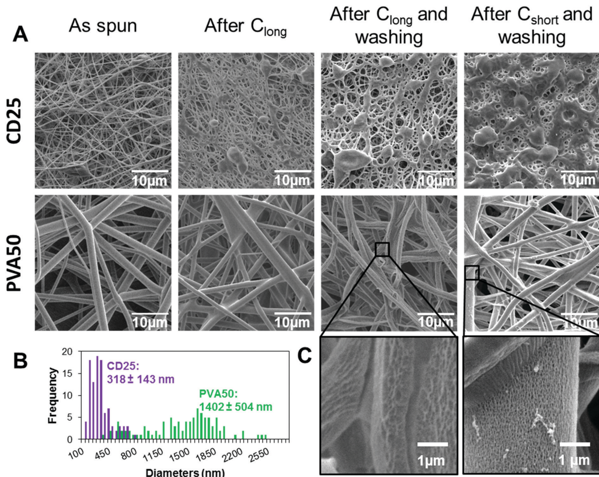
Fig. 3 Morphology of the fibers as spun and after post-treatments. Low magnification SEM pictures (A), diameter distribution of diameters of as-spun fibers (B) and high magnification pictures of cured PVA50-washed fibers (C). CD25 contains 50% of PGS, 25% of HP \beta CD and 25% of PVP; PVA contains 50% of PGS and 50% of PVA. The morphology is shown here after C_{long} (24 h at 120 °C, 48 h at 140 °C and 24 h at 170 °C) and after 24 h washing in water.
