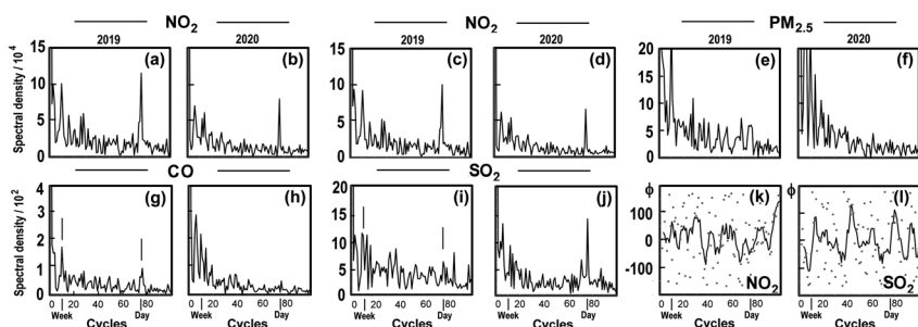
Fig. 3 Fourier transforms of hourly concentration data across Beijing for 75 days starting on 24th January: (a) NO_2 2019 within 5th Ring Road 2019, (b) NO_2 2020 within 5th Ring Road and across all the sites 2019, (c) NO_2 , (d) NO_2 , (e) PM_{2.5} 2019, (f) PM_{2.5} 2020, (g) CO 2019, (h) CO 2020, (i) SO_2 2019 and (j) SO_2 2020, and the phase angle, in degrees for (k) NO_2 within 5th Ring Road 2020 and (l) SO_2 2020, where the smoothed trend line added is a 5-point running mean. Note: the x-axis shows the number of cycles in the 75 day record, so 75 marks the daily cycle, and the weekly cycle is expected at 10–11 as marked. The y-axis in figures (a)–(j) denotes spectral power which takes the units of concentration squared. The y-axis in figures (k) and (l) is the phase angle in degrees.
