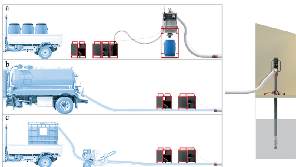
Fig. 4 The Excluder (right) can be linked to a) a custom vacuum system (Flexclevator), b) vacuum truck, or c) a pit-side pump.
