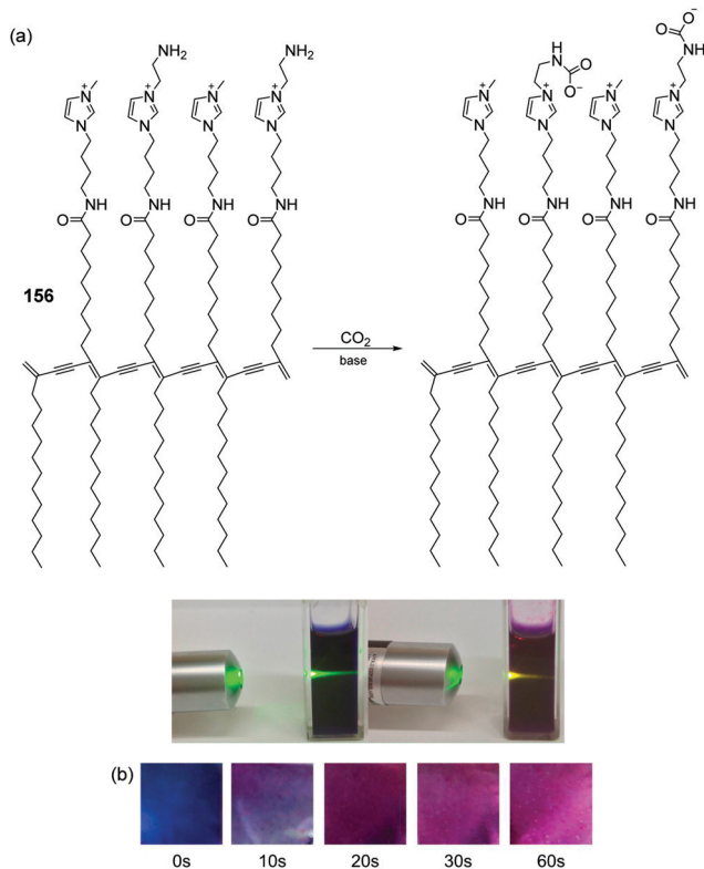
Fig. 15 (a) Structure of 156 , and proposed origin of the CO 2 induced color change. (b) Time-dependent color changes of 156 embedded in electrospun microfibers in a CO 2 atmosphere in the presence of saturated TEA vapor.
